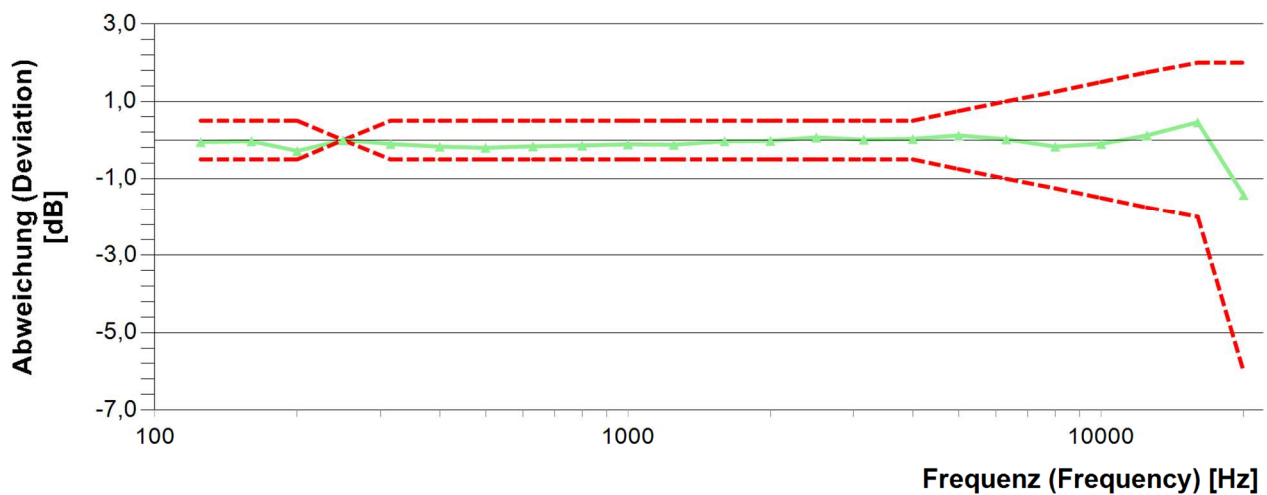
Diagramm Amplitudenfrequenzgang Amplitude frequency response graph
